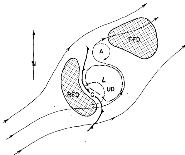
FIG. 10. Storm-relative flow at mid-levels (~7 km) after stage 2 of supercell evolution. The thick barbed line is a strong temperature and vertical velocity interface; updraft (UD) is finely stippled and downdraft, both the forward flank (FFD) and rear flank (RFD), is coarsely stippled. The L is the core of the original mesocyclone and C is the center of the transformed or divided mesocyclone. The A indicates a region of anticyclonic vorticity.
