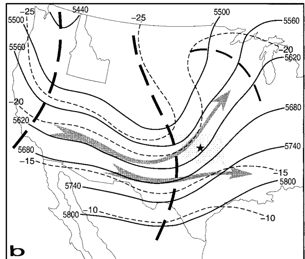
FIG. 6. The 500-mb analyses as in Fig. 5 for (a) 1500 UTC on 25 Mar 1948 and (b) 0300 UTC on 26 Mar 1948.
