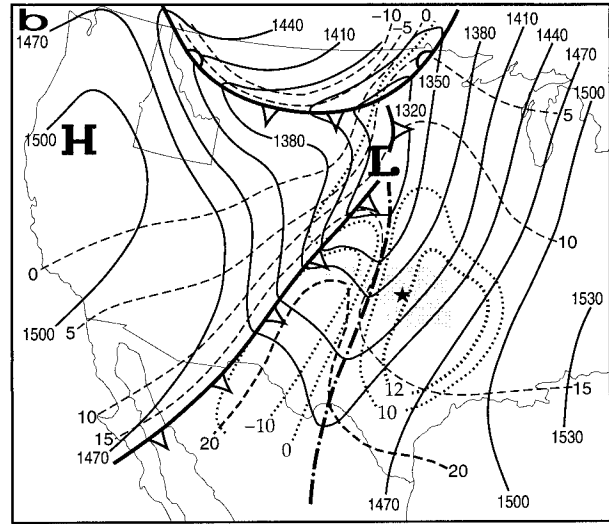
FIG. 4. The 850-mb analyses as in Fig. 3 for (a) 1500 UTC 25 Mar 1948 and (b) 0300 UTC 26 Mar 1948.
