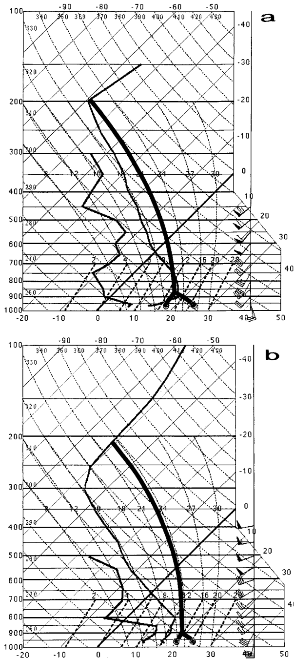
FIG. 8. Skew T - \log p plots of the Oklahoma City soundings at 1500 UTC on (a) 20 Mar 1948 and (b) 25 Mar 1948. Winds are full barb for 10 kt (or 5 \text{ m s}^{-1} ) and flags for 50 kt (or 25 \text{ m s}^{-1} ). The surface parcel and its lifted characteristics are indicated for the maximum concurrent observed values of temperature and dewpoint prior to the tornadoes.
