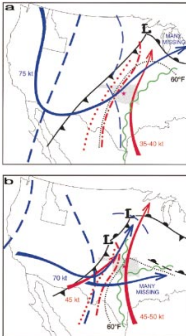
FIG. 7. Composite charts constructed for (a) 0600 UTC 21 Mar 1948 and (b) 0000 UTC 26 Mar 1948. Features are as on preceding charts with 500-mb features in blue, 850-mb features in red and green, and surface frontal analyses and 60°F dewpoint in black. The wavy green lines indicate moisture axes at 850 mb and the red dotted lines the axes of highest temperatures at 850 mb. Maximum observed wind speeds are indicated; many winds were missing at 500 mb.
