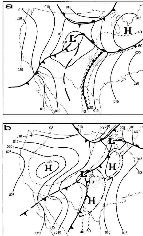
FIG. 1. Surface analyses for (a) 1230 UTC 20 Mar 1948 and (b) 1230 UTC 21 Mar 1948. Isobars are shown at 5-mb intervals. The dryline (continuous round blips); surface troughs (heavy dashed lines); 20°, 40°, and 60°F dewpoint isodrosotherms (dashed lines); squall lines (dash-double dot lines); and standard surface analysis features are shown. The location of Tinker AFB is indicated by the star.
