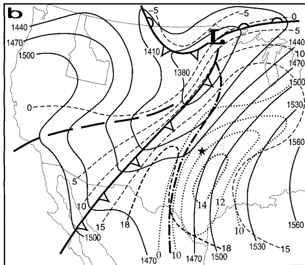
FIG. 3. The 850-mb analyses for (a) 1500 UTC 20 Mar 1948 and (b) 0300 UTC 21 Mar 1948. Symbology follows Miller (1967). Fronts are shown with open bars. Height troughs are heavy dashed lines. Dryline positions are heavy dash-dot lines. Temperature (dewpoint) isotherms (isodrosotherms) are light, dashes (dots) in ^{\circ}\text{C} . Height contours are in m.
