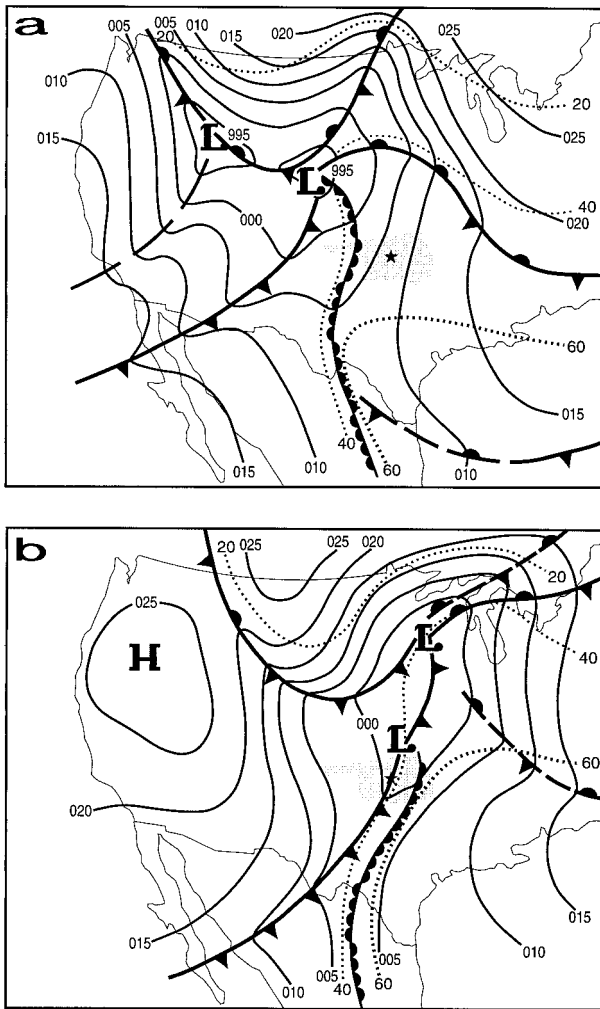
FIG. 2. Surface analyses as in Fig. 1 for (a) 1230 UTC 25 Mar 1948 and (b) 1230 UTC 26 Mar 1948.
