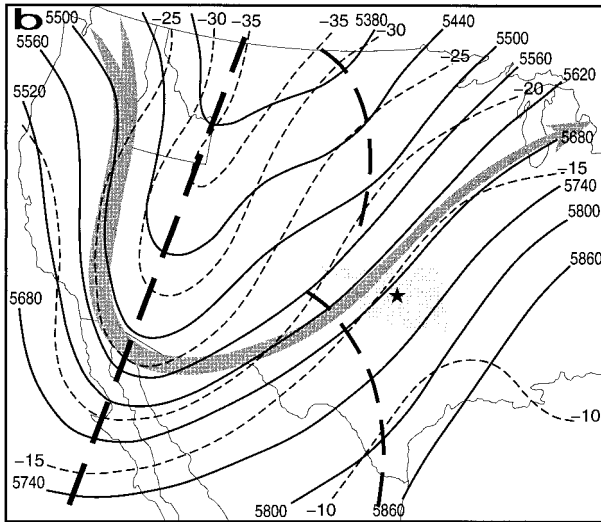
FIG. 5. The 500-mb analyses for (a) 1500 UTC 20 Mar 1948 and (b) 0300 UTC 21 Mar 1948. Height contours are in m. Major height trough positions are heavy dashed lines, and minor troughs are lighter dashed lines. Isotherms in °C are light dashed lines. The axis of strongest wind speeds is indicated by gray-shaded arrow.
