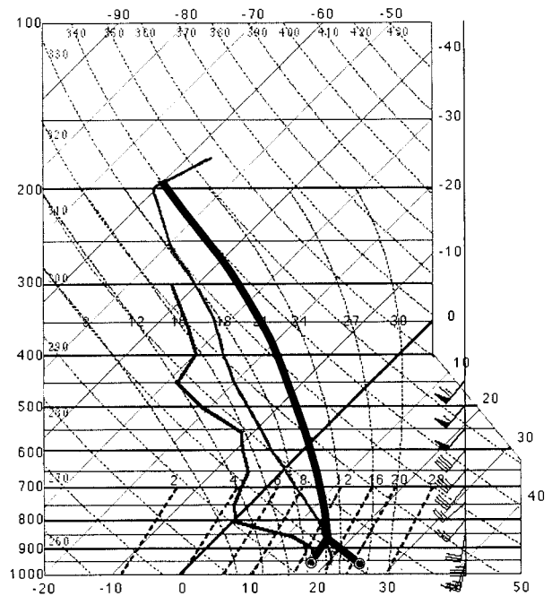
FIG. 9. Skew T - \log p plot of the Oklahoma City sounding for 0300 UTC on 21 Mar 1948. Details as in Fig. 8.
