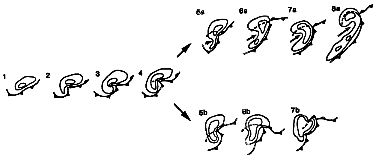
FIG. 4. Schematic showing two different paths of evolution with HP supercells, adapted from Moller et al. (1990). The low-level reflectivity patterns are shown as thin solid lines, and the associated outflow boundaries are depicted with frontal symbols. The "a" sequence (upper right) shows the rear downdraft/outflow with small arrows.
